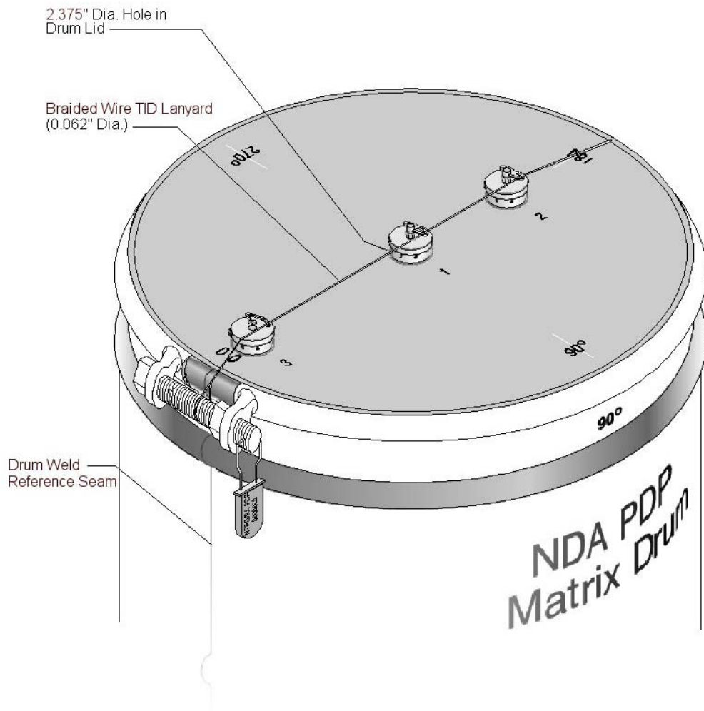
Figure F-7. NDA PDP matrix drum sample TID mechanism.
